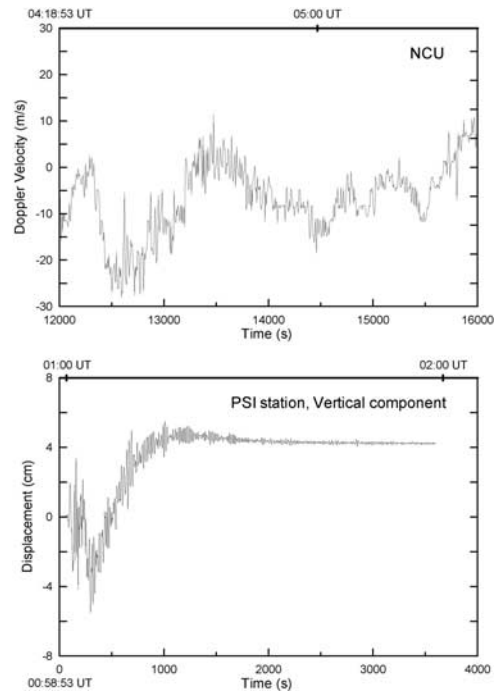
Figure 3. (top) Enlarged portion of the Doppler sounder record obtained at NCU, showing a big pulse of 30-minute duration. (bottom) Vertical ground displacement record obtained at the broadband seismic station PSI, showing a big transient followed by a permanent uplift of about 4 cm.
