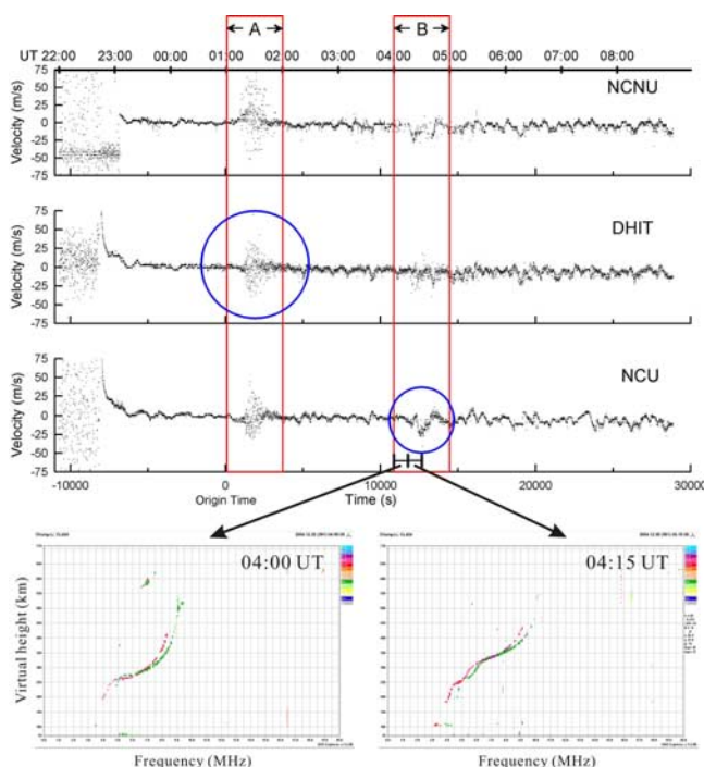
Figure 2. (top) Digital Doppler sounder records of the ionospheric disturbance obtained at stations NCNU, DHIT, and NCU. The circled portions of NCU and DHIT are enlarged in Figures 3 and 4, respectively. (bottom) Ionosonde records obtained at station HSS at 04:00 UT and 04:15 UT.
