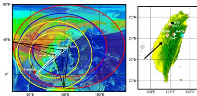
Figure 1. (left) Locations of the epicenter (red star) and fault rupture area (black box) of the M9.3 Sumatra earthquake, the broadband seismic station PSI, and the ionosonde stations HSS (24.7°N, 121.0°E; 3580 km to the epicenter), YAM (31.7°N; 130.6°E, 4810 km), and KOK (35.9°N; 140.1°E, 5800 km). The possible distance to the source from HSS (yellow rings), YAM (blue rings) and KOK (red rings). (right) Observational sites in Taiwan, including the ionospheric reflection points of the digital Doppler sounder receiving stations NCNU (24.1°N; 120.8°E), DHIT (24.2°N; 121.2°E), and NCU (24.7°N; 121.0°E), digital ionosonde station HSS, and broadband seismic station NACB.
