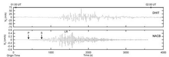
Figure 4. (top) Enlarged portion of the Doppler sounder record obtained at DHIT, showing oscillatory ionospheric disturbances. (bottom) Time histories of the vertical ground velocity obtained at NACB. The arrival times of P, S, and LR (Rayleigh) waves are marked on the trace.
